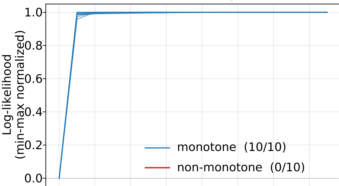
(theorem respects)
